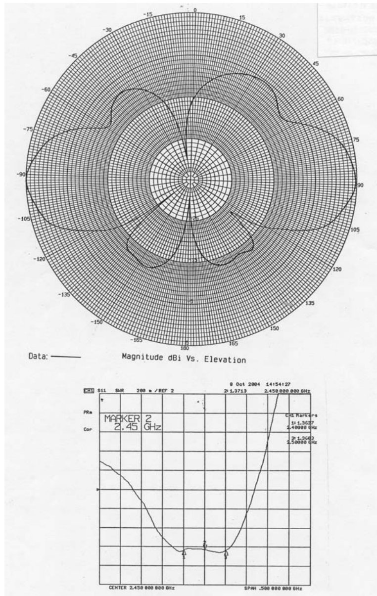
ECO5-2400 Series – Elevation Plot
